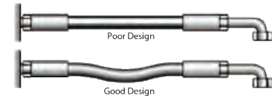
FIGURE 3 Hose length should allow for the flexing of hose when there is contraction and expansion during use.
