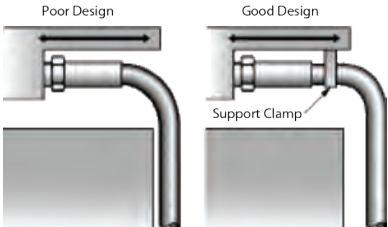
FIGURE 6 Support clamps are a good tool to use when trying to limit hose wear due to abrasion. Clamps can be used to isolate hose and hold them away from abrasive surfaces or environments.
