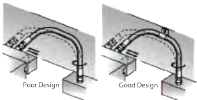
FIGURE 5 The proper use of clamps can help relax the hose when there is movement in more than one plane. Caution must be taken to use the correct clamp so the cover of the hose is not damaged and to provide enough length of hose on either side of the clamp to allow for movement.
