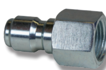
14-0390 QC 3/8" FNPT ZINC STEEL PLUG
